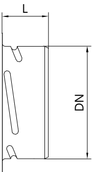
KM mounting collar
