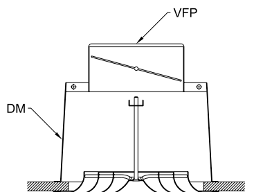
Installation with the use of DM plenum box with VFP damper
